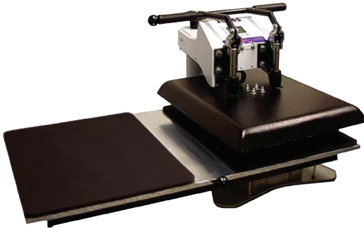
HP-DK20S-TWIN Twin Shuttle Attachment
